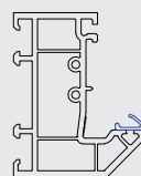
701501 56mm Outerframe
