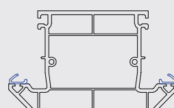
702505 116mm Midrail
