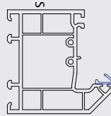
701502 72mm Outerframe
