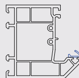
701502 72mm Outerframe
