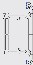
702152 116mm Patio Midrail Bevelled
