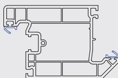
705510 110mm Door Sash Open In
