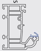
701531 56mm Outerframe
