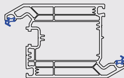
103366 115mm Open In Door Sash/Z Midrail
