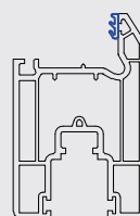
705151 90mm Patio Sash Bevelled
