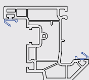
703509 79mm Tilt & Turn Sash
